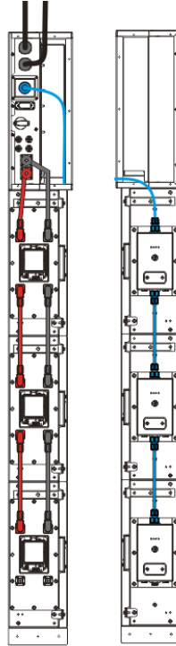
Figure 7-2 Installation Diagram
