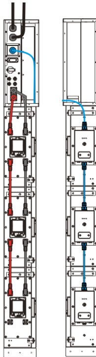
Figure 7-7 Single Phase All-in-one System Connection Schematic
